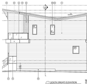
SOUTH (RIGHT) ELEVATION
