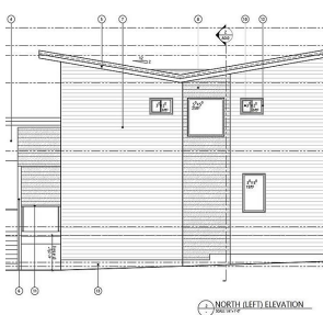
NORTH (LEFT) ELEVATION
