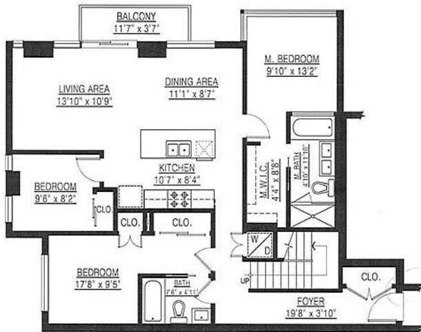
MAIN FLOOR PLAN FLOOR AREA: 1,145 sq.ft.
